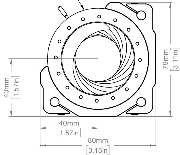
ADJUSTABLE IRIS DIAPHRAGM Ø 69.85mm [Ø 2.75in]
