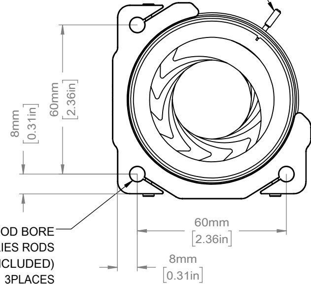
IRIS APERTURE ADJUSTMENT LEVER Ø 0.8mm [Ø 0.03in] MINIMUM APERTURE Ø 50.0mm [Ø 1.97in] MAXIMUM APERTURE
