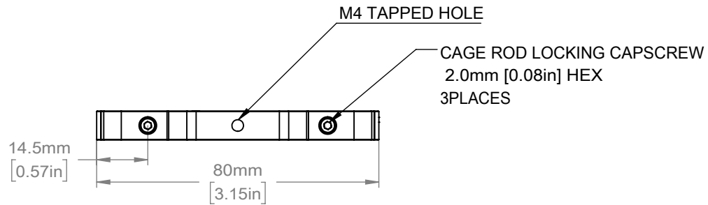
ADJUSTABLE IRIS DIAPHRAGM Ø 69.85mm [Ø 2.75in]
